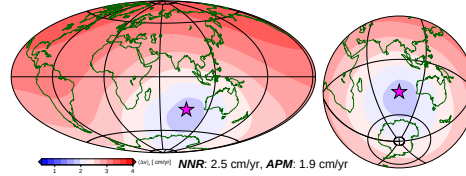
e) ridge no mot. (92.8°, -35.5°, 0.167 °/Myr)
