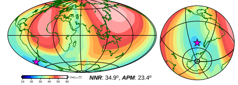
c) spr. align., Pacific (262.6°, -49.0°, 0.629 °/Myr)
