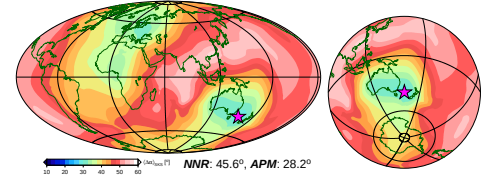
i) SKS (158.9°, -40.1°, 0.720 °/Myr)
