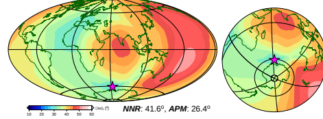
a) spread. align. (63.9°, -61.2°, 0.277 °/Myr)
