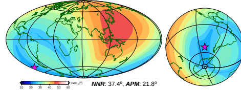
d) spr. align., Indian (256.1°, -48.8°, 0.164 °/Myr)
