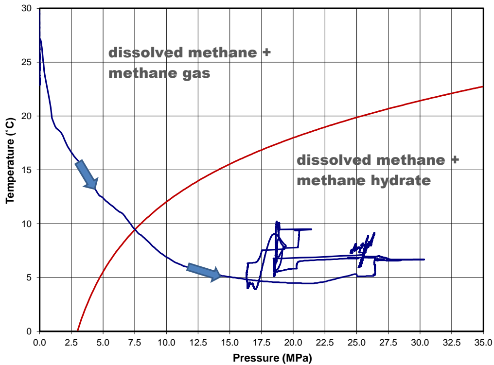
UT-GOM2-1-H005-13FB Rabbit P vs T
