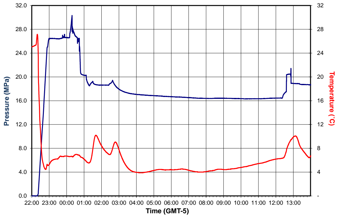
UT-GOM2-1-H005-13FB Rabbit PT record 20 May 2017
