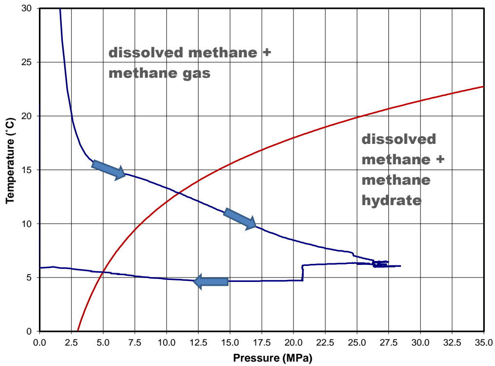
UT-GOM2-1-H005-12FB Plug P vs T
