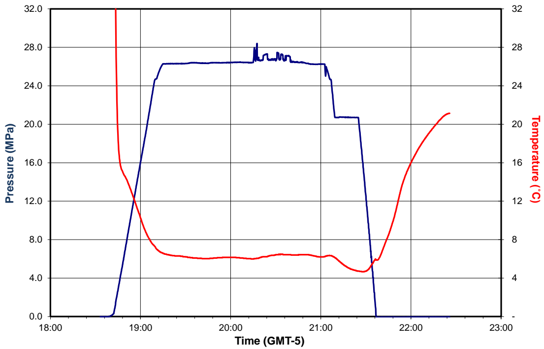
UT-GOM2-1-H005-12 FB Plug PT record 12 May 2017
