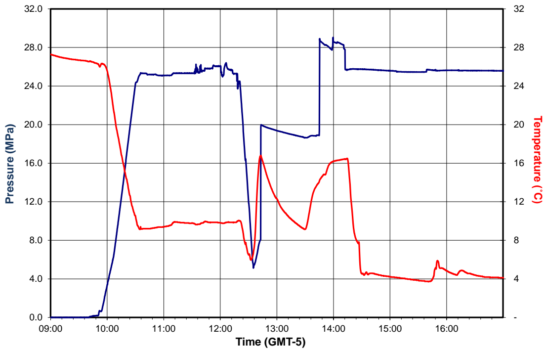
UT-GOM2-1-H005-2FB Plug PT record 18 May 2017
