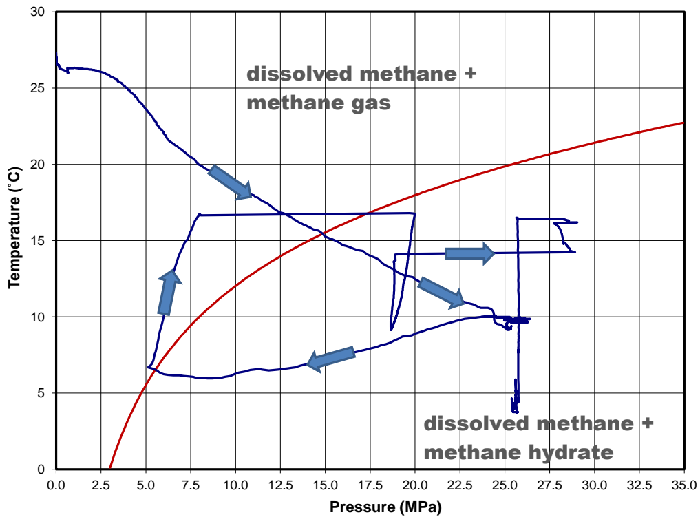
UT-GOM2-1-H005-2FB Plug P vs T
