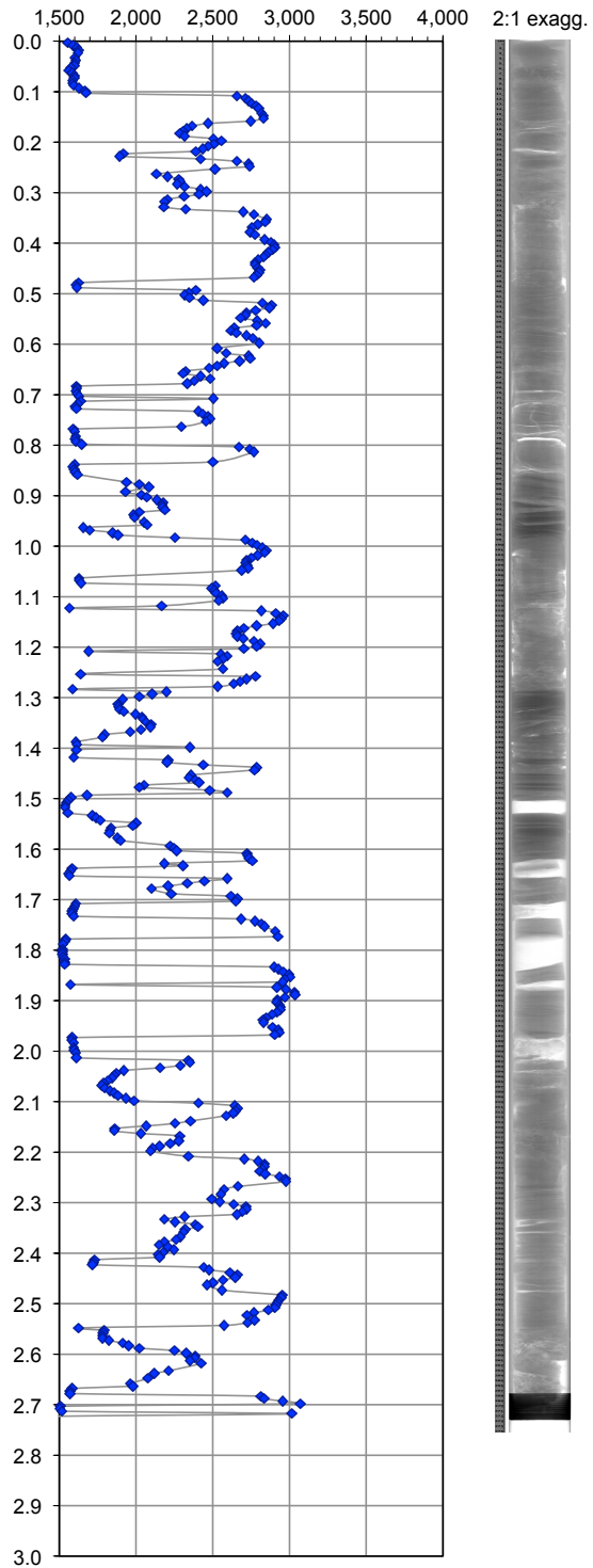
P-wave Velocity (m/s)
