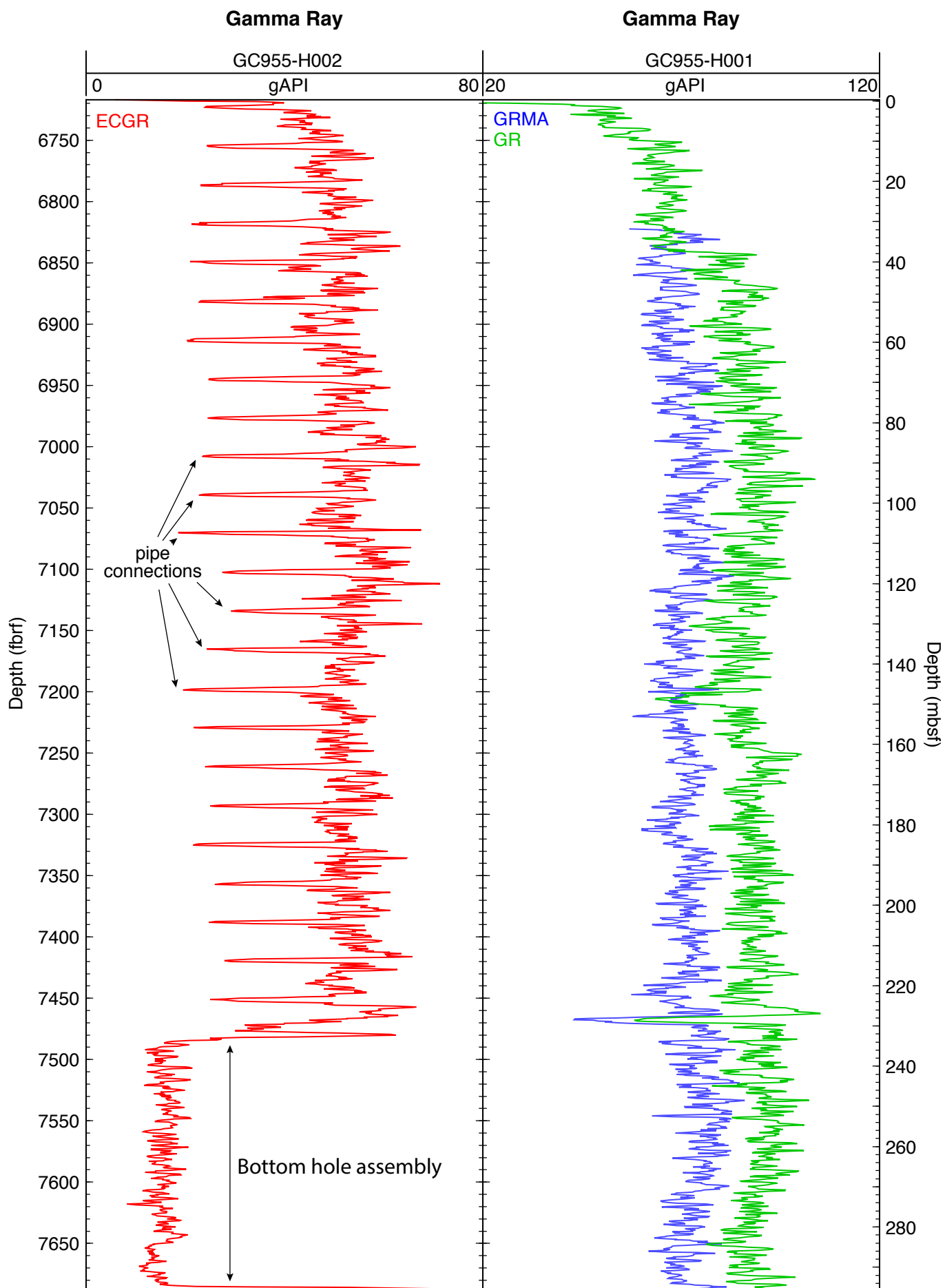
Figure 3.8.5 – GR in pipe and comparison with GC955H
