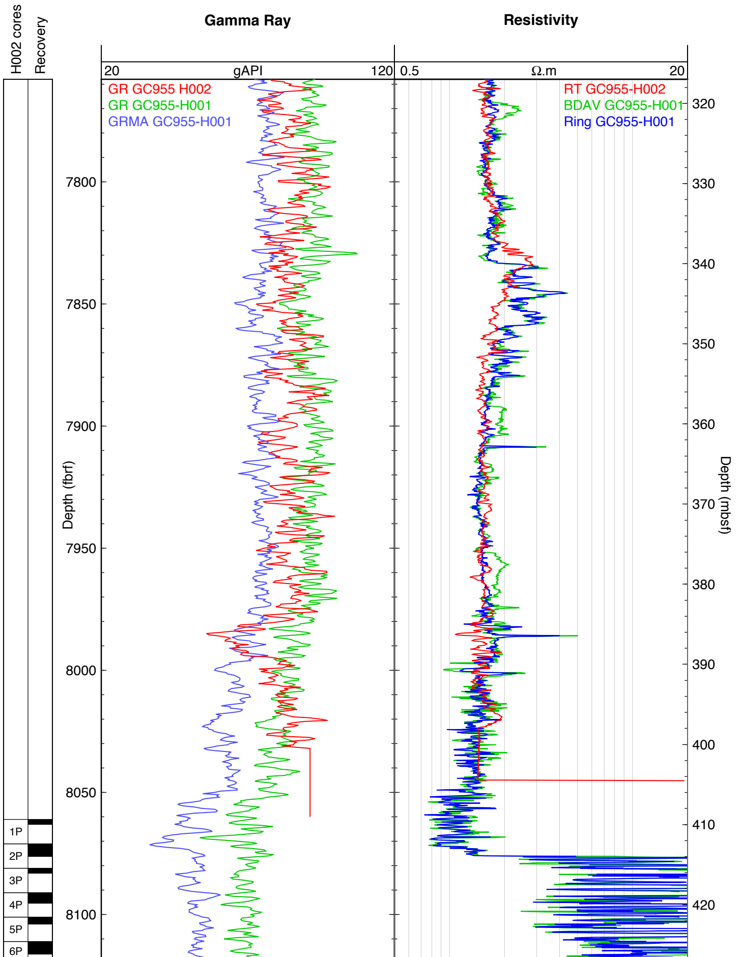
Figure 3.8.4 – Comparison with GC955H
