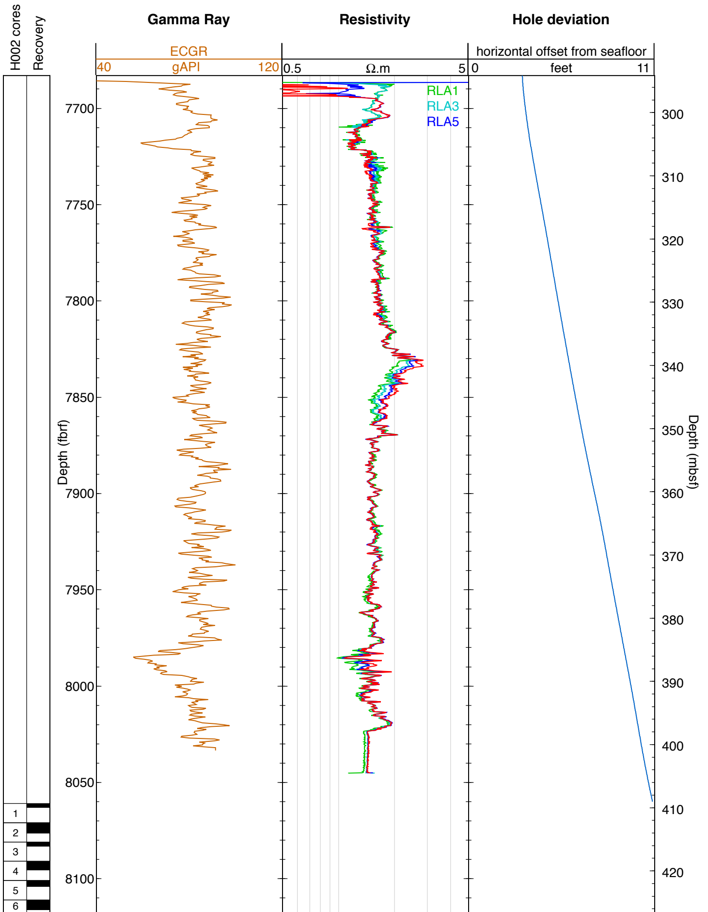
Figure 3.8.2 – Summary of logs in open hole
