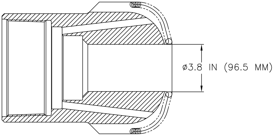
PCTB CUTTING SHOE CONFIGURATION DRILL BIT
