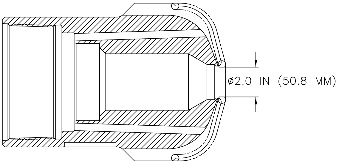
PCTB FACE BIT CONFIGURATION DRILL BIT
