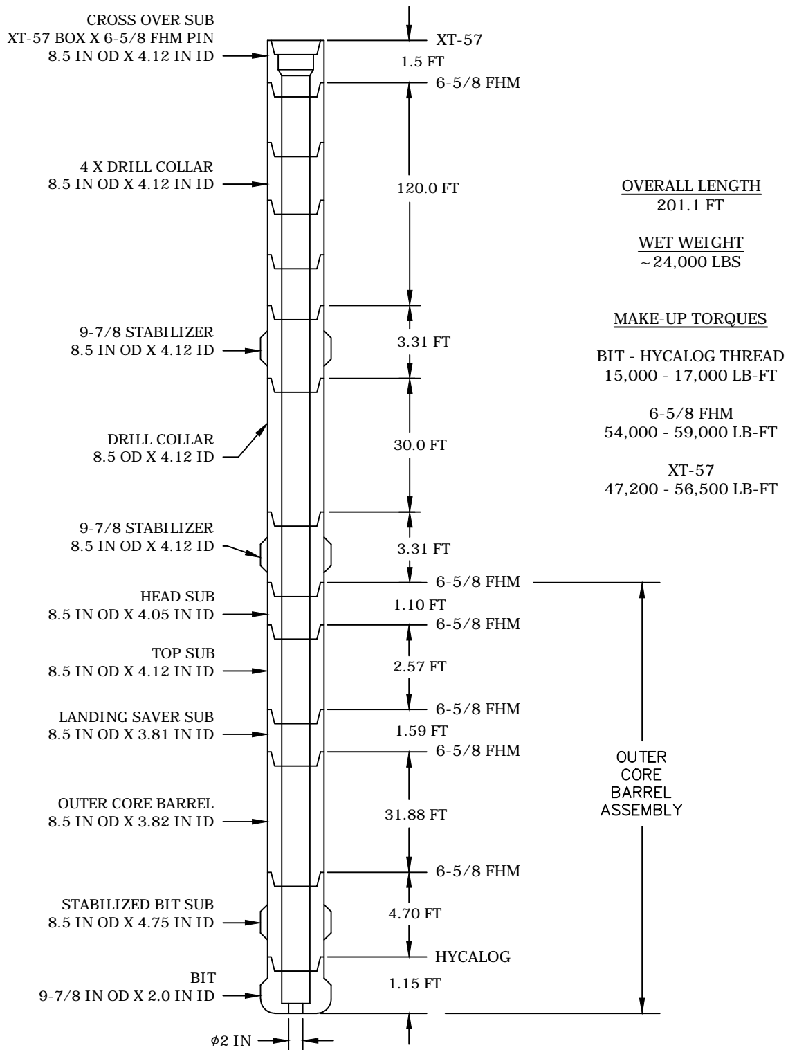
PCTB FACE BIT CONFIGURATION BHA SCHEMATIC
