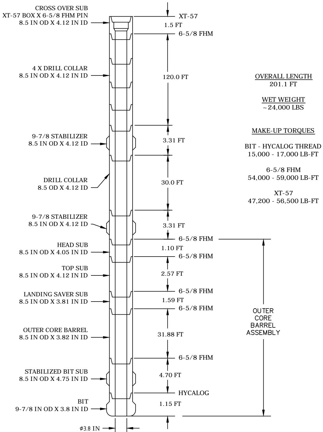
PCTB CUTTING SHOE CONFIGURATION BHA SCHEMATIC
