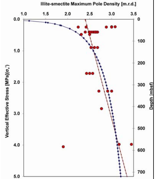
Fig. 1: Illite-smectite preferred orientation of Ursa mudstones as a function of vertical effective stress. Straight line is a simple linear model predicting Illite-smectite preferred orientation from vertical effective stress. Curved line incorporates void ratio into the prediction of preferred orientation.
