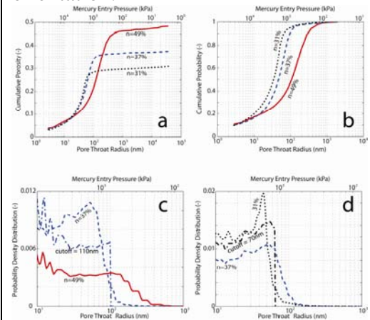
Fig. 2: Close off model for pore throat size distribution
