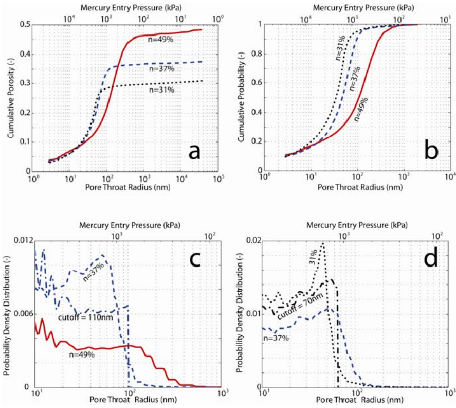
Fig. 2: Close off model for pore throat size distribution
