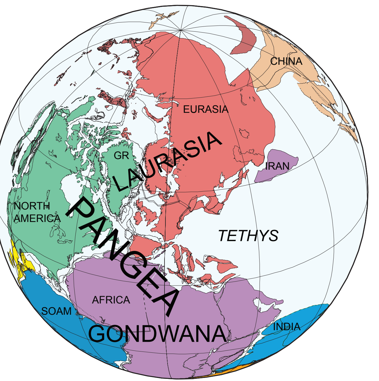
200 Ma Late Triassic
