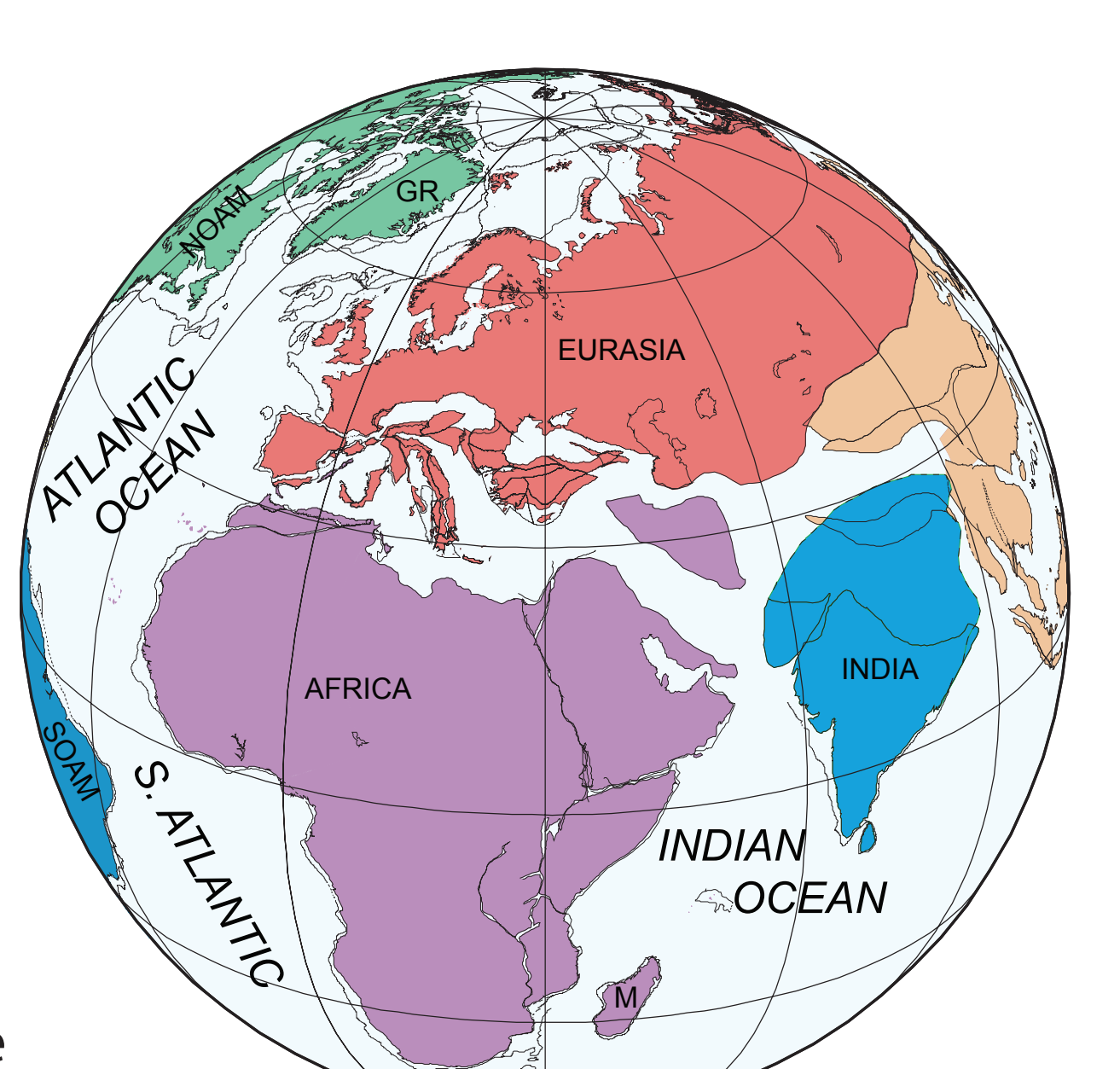
40 Ma Middle Eocene
