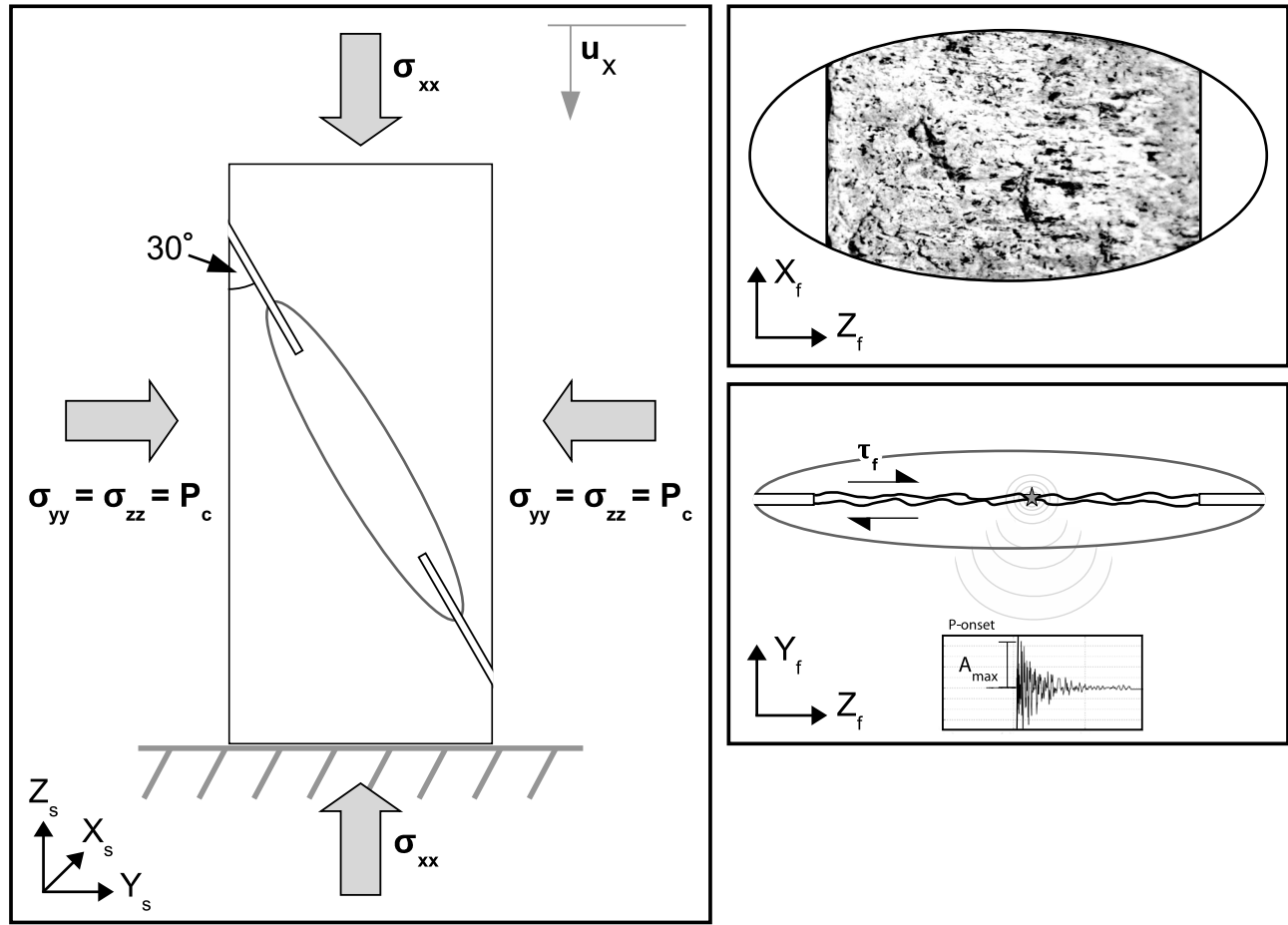
Figure 1. (left) Schematic diagram of loading conditions and stresses. Arrows at bottom left specify the sample-specific coordinate system. (right) Sliding of fault with naturally developed roughness in fault specific coordinate system which is also used for the later AE representation.
