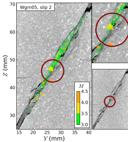
Figure 13. CT scan of central part of sample obtained after the experiments and AE hypocenters (colored dots) for the stick periods before slip event 2 of WGRN05. The colors of hypocenter locations correspond to their magnitudes. The red circle highlights the likely site of a large asperity which was centered at [27,45].
