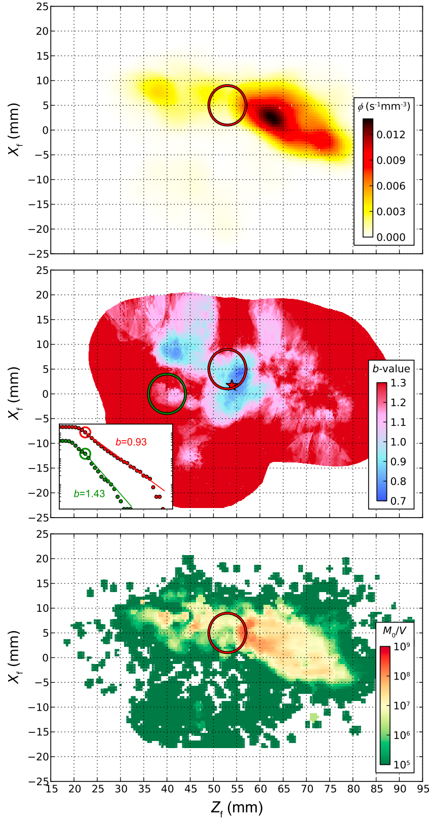
Figure 10. Examples of AE event density ( \phi ), b value and moment release maps computed for AEs occurring before slip event 1 of experiment WGRN05. Slip event one (red star) nucleated close to or from within an area of high \phi , M_0 and low b value. The finds for high and low b value regions are compared (bottom left in Figure 10 (middle)). The asperity region is connected to low b values, high event density and moment release.
