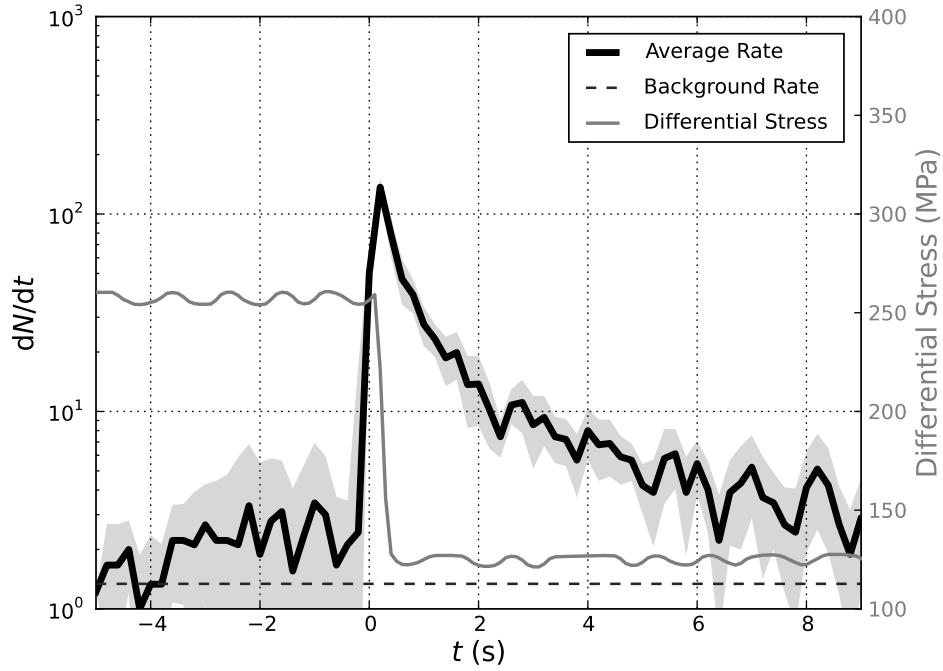
Figure 4. Differential stress (gray line), AE rate average (black line), standard deviation (shaded gray region), and background rate (dashed gray line) for all slip events of WGR01, WGRN04 and WGRN05 within a 15 s time window of slip onsets, stacked to t = 0 . The origin times of slip events were determined from the stress drop onsets and compared to AE data. The highest AE rates occurred within less than 100 \mu s of the stress drops.
