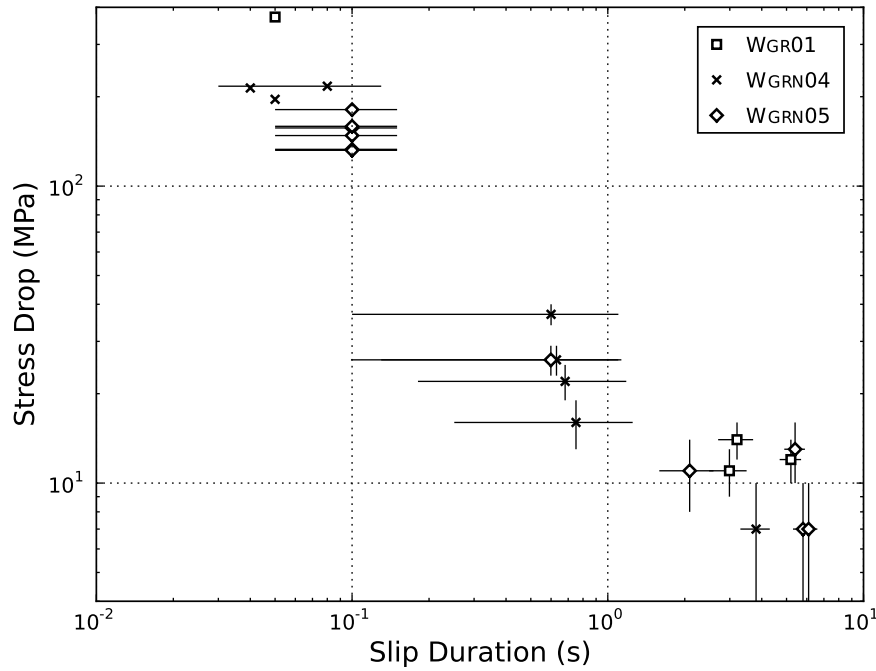
Figure 6. Stress drop ( \Delta\sigma ) and duration of slip events for three different samples. Vertical errors represent uncertainties in stress measurements while horizontal uncertainties are estimated errors for onset picks of stress drop start and end which are larger for small stress drops due to a smaller signal to noise ratio. Slip events with large stress drop had a maximum duration of 0.1 s. Decreasing stress drops were connected to increasing slip durations of up to 6 s. The duration uncertainty for all large stress drops was 0.1 s while low stress drop events had estimated uncertainties of 0.5 s.
