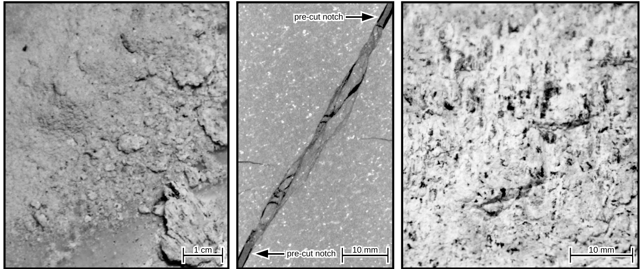
Figure 5. (left) Photo of gouge, which was produced within the fault zone during the 6 stick slips of WGRN05, consisting of ultrafine and larger grains. Larger rock flag at bottom right shows evidence of slickensides and black elongated grains as a result of slip under high normal stress. (middle) CT image of the fault structure with scale in mm after the completion of the experiments. The fault width and gouge layer thickness varied along the fault. (right) Photo of fault surface with many slip-parallel slickensides and topographic relief changes of up to 2 mm.
