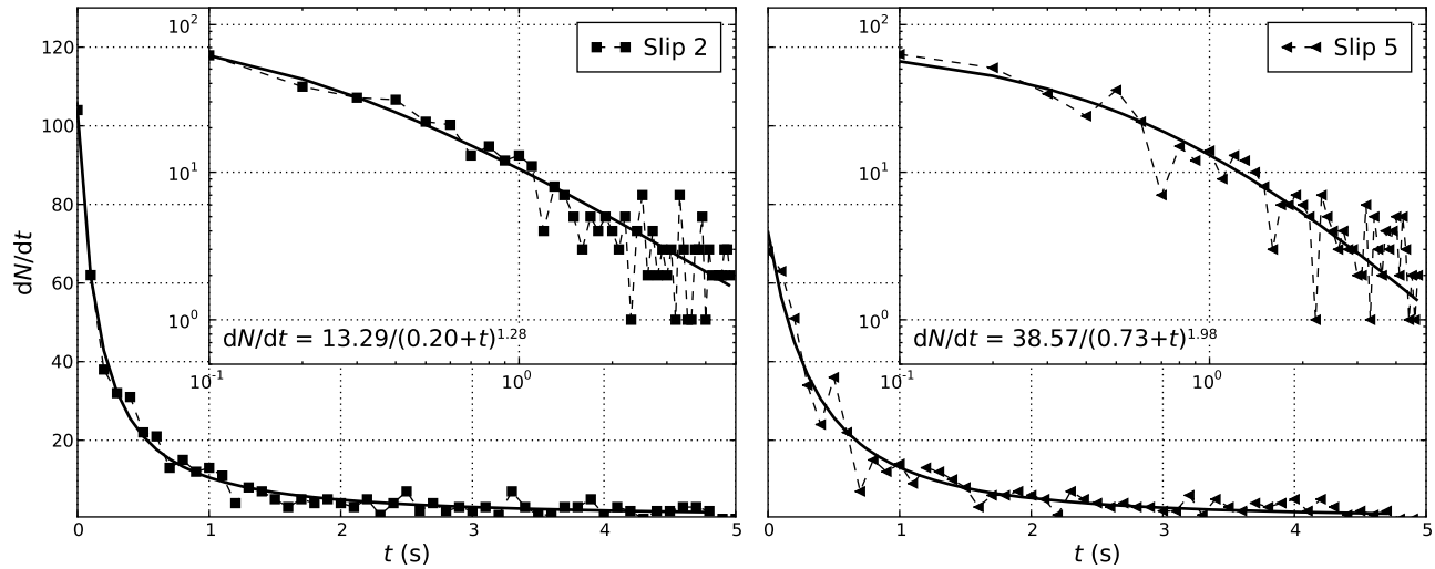
Figure 7. AE aftershock rates for slip events 2 and 5 plotted in linear and logarithmic scale.
