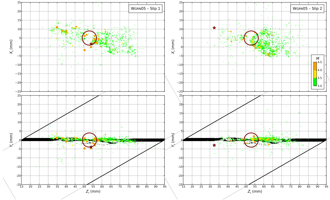
Figure 9. Examples of AE foreshock activity based on slip events 1 and 2 of WGRN05. The red circle highlights an area of a relatively sharp contrast between low and high AE activity. Many large amplitude events were produced in the periphery of this area before each of the slip events.
