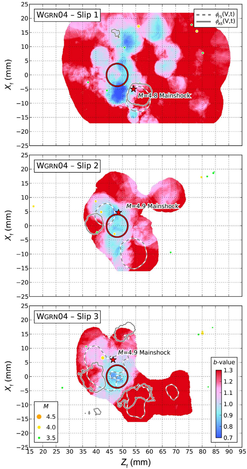
Figure 12. b value, foreshock and aftershock densities, main and largest aftershock locations plotted similarly to Figure 11 but now for three different slip events of experiment WGRN04. A combination of b value maps, AE event densities and foreshock locations enables the identification of an asperity region (red circle) which is also the nucleation spot of macroscopic slip events.
