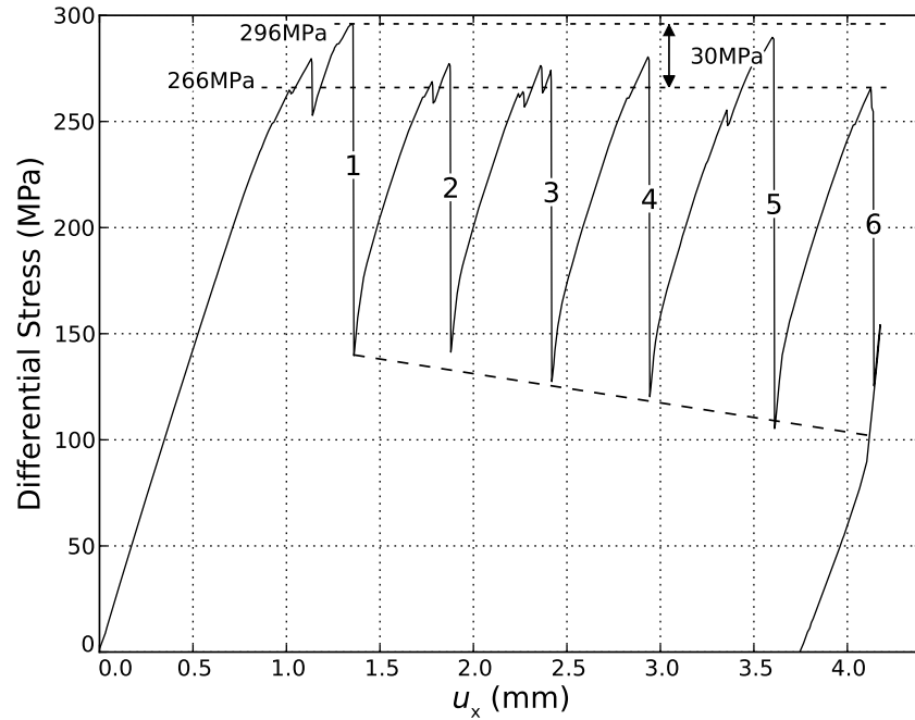
Figure 2. Differential stress and axial displacement ( u_x ) for experiment WGRN05 with characteristic stick-slip behavior. The slip events with large stress drops are labeled from 1 to 6. All slip events with large stress drops nucleated within a differential-stress window of 30 MPa (dashed lines at top). The residual stress decreased systematically after each successive stick slip as indicated by the downward sloping dashed line.
