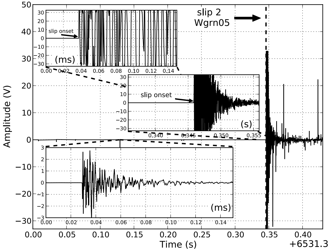
Figure 3. AE waveforms within a \sim 0.5 s (main axis), 20 ms (middle) and 0.15 ms (inset at top) time window of slip event 2 of experiment WGRN05 as well as a waveform of a “typical” AE event (inset at bottom). The waveforms connected to slip onsets were clearly distinguishable from commonly observed AEs by their amplitude and duration. Note that time scales are in ms for the top and bottom insets.
