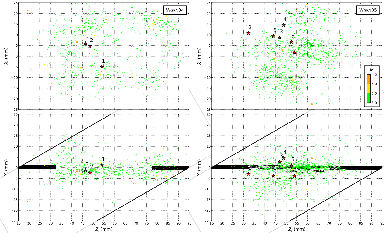
Figure 8. Figure 8 (top) shows AEs (main shocks and aftershocks) projected onto fault plane; Figure 8 (bottom) images AEs within a plane normal to the fault for samples (left) WGRN04 and (right) WGRN05. The red stars indicate the location of the large amplitude AEs coinciding with the onset of the stress drops for all slip events. Dots are aftershocks to slip events colored by size. The nucleation points of stick-slips cluster within similar regions for individual experiments except for event 2 of WGRN05.
