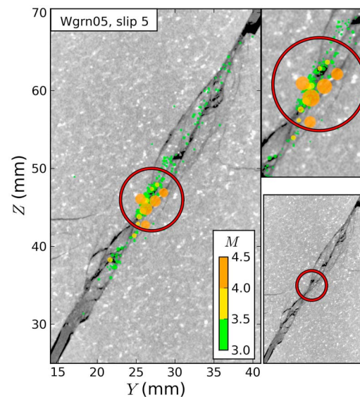
Figure 14. CT scan and AE hypocenters colored according to magnitude for foreshocks to slip event 5 of WGRN05. Most of the AE activity is concentrated within the asperity region indicated by a red circle.
