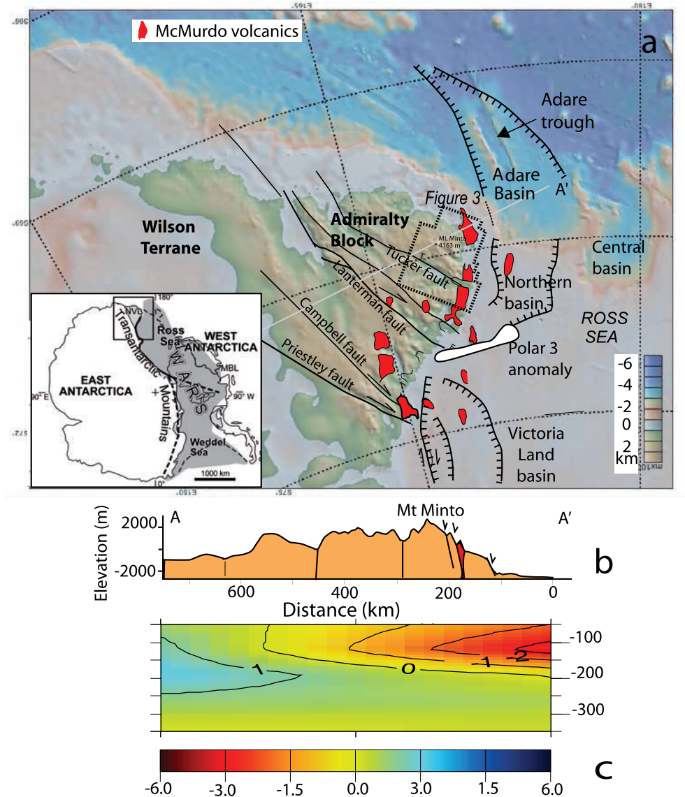
Figure 1. (a) Tectonic map of the Ross Sea region with main structural features and distribution of McMurdo volcanics (modified after Salvini et al. [1997], Cande et al. [2000], Davey and De Sanctis [2005], and Davey et al. [2006]). The inset shows the Antarctic continent and the West Antarctic Rift system (WARS). Location of the study area is shown. MBL, Marie Bird Land; NVL, north Victoria Land. (b) Cross-section AA' shows the main structural architecture across NVL and their relationships with topography and magmatism along with (c) the corresponding upper mantle DM01 model [Danesi and Morelli, 2001] tomographic section (see Figure 2).
