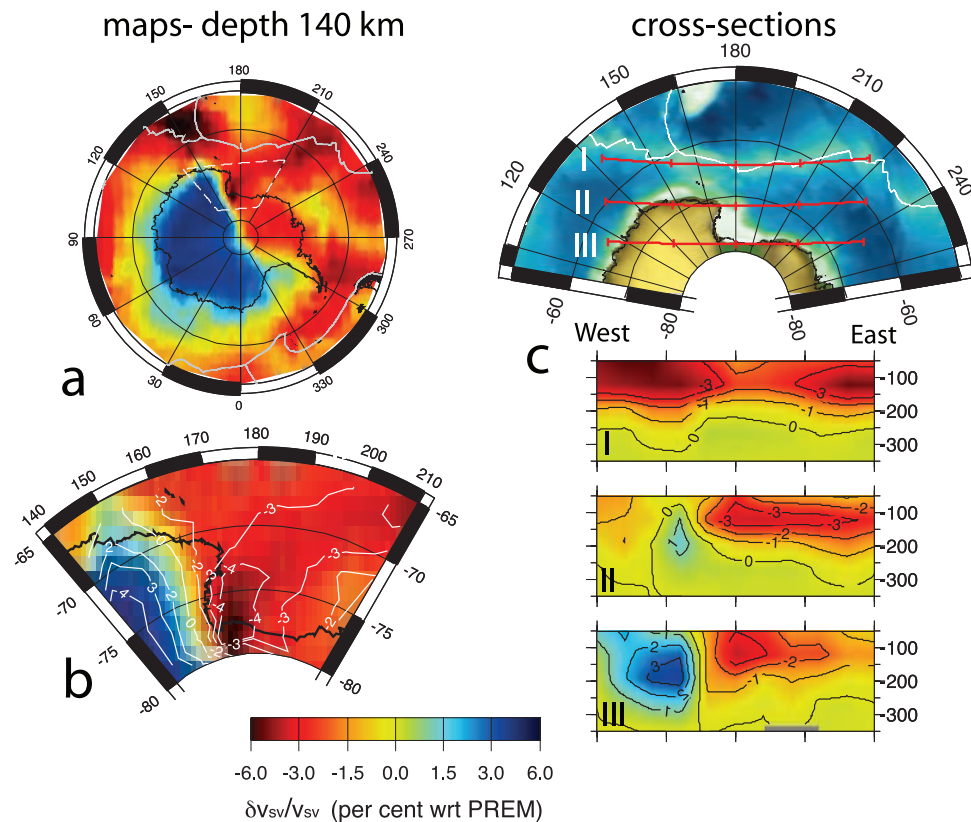
Figure 2. Maps of the shear wave velocity variations in DM01 model [Danesi and Morelli, 2001] at 140 km depth beneath (a) entire Antarctica and (b) Northern Victoria Land (dashed white line in Figure 2a). Color scale represents percent variations with respect to anisotropic PREM (Saturated blue regions beneath the East Antarctica shield are about 6% faster than PREM). (c) Cross sections show the velocity distribution down to 350 km depth (see location on the top map). Section I crosses the Tasman-South Pacific Ridge, close to the triple junction (note saturated red areas correspond to v_{sv} 5–6% slower than predicted by PREM). Section II crosses the North Victoria Land (study area) close to the craton edge. Section III crosses the sharp discontinuity between the East Antarctica shield and the Ross Sea Embayment. Note warm (slow) anomalies beneath Ross Sea and ocean ridges, and cold (fast) lithospheric roots underneath the Archean shield of East Antarctica.
