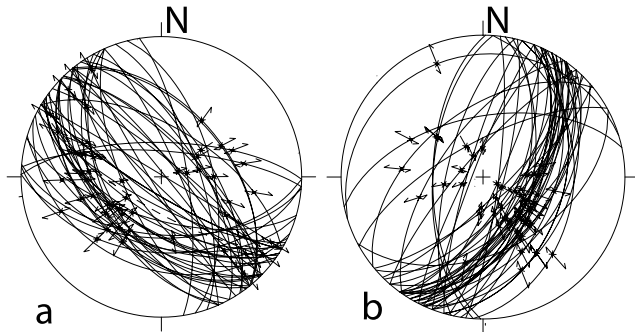
Figure 4. Stereonets (Schmidt net lower hemisphere) showing the trace of fault planes and slickenlines related to the (a) first and (b) second episode of brittle deformation (fault as great circles, slickenlines as arrows).
