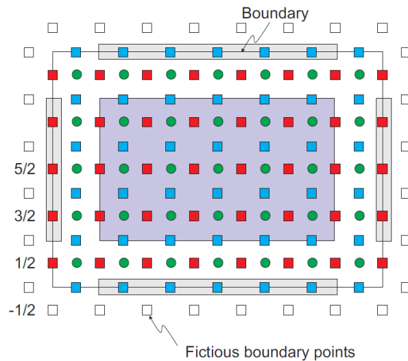
Figure 4.19: Staggered grid definition with the boundary points. Within the purple domain, the finite difference scheme for center points can be applied. At the boundaries, we have to apply a special finite difference scheme which employ fictitious boundary nodes.
