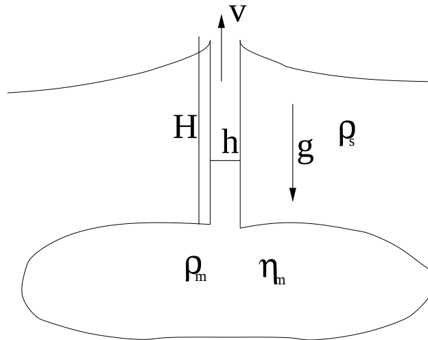
Figure 2.4: Illustration of the geometry of the volcanic eruption problem.
