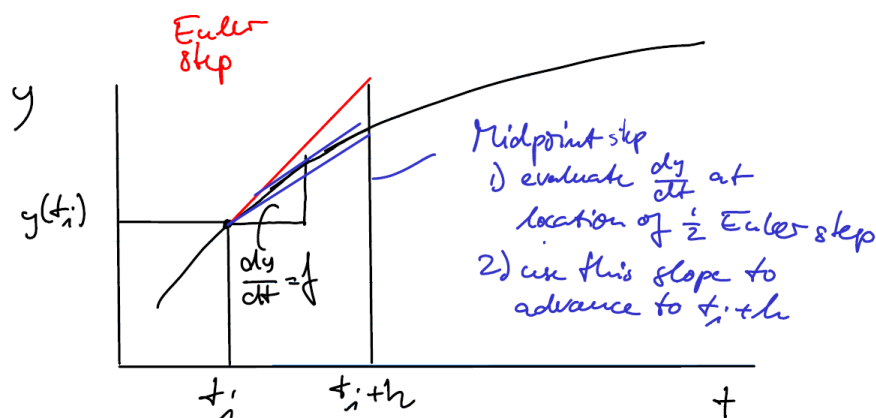
Figure 3.2: Sketch illustrating the midpoint method.
